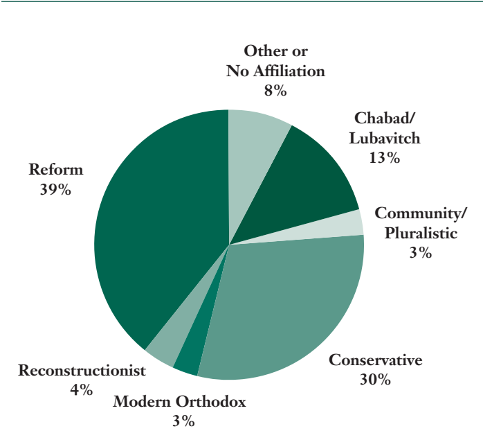
GRAPH 2: SCHOOL AFFILIATION
